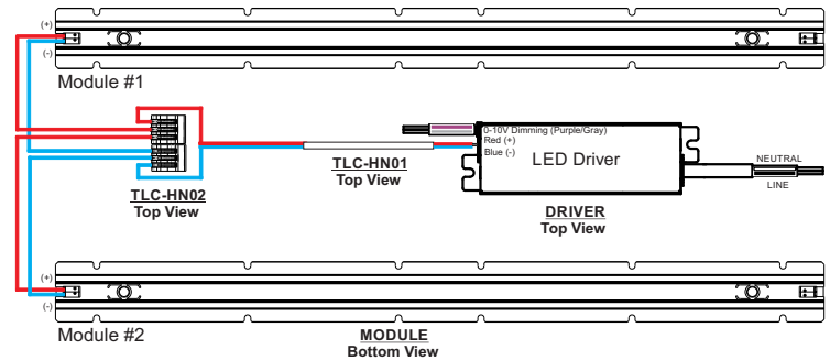
Two Module Wiring (4P, DRIVER WITH CONNECTORS)
