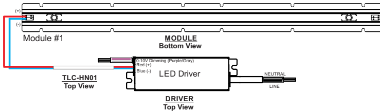
One Module Wiring (3P, DRIVER WITH CONNECTORS)
