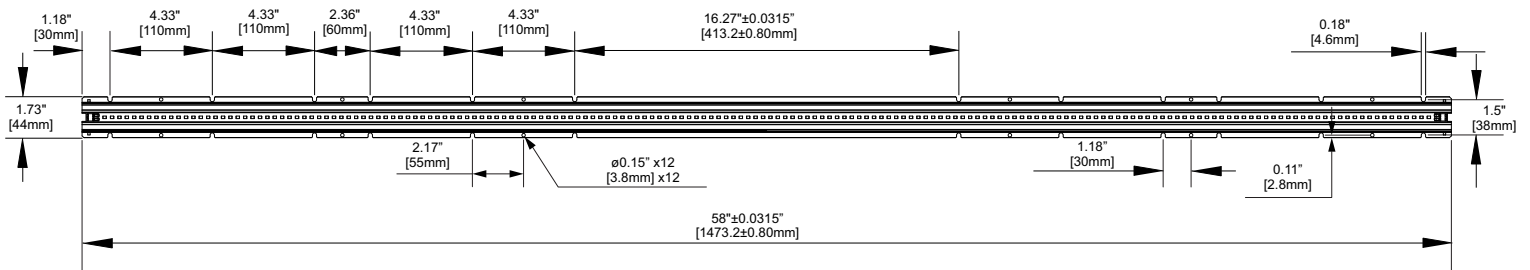
TOP VIEW
