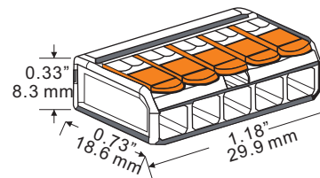
ISOMETRIC VIEW
