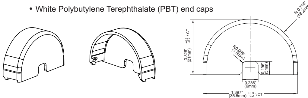
ISOMETRIC VIEW
