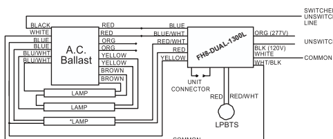
5. THREE LAMP RAPID START BALLAST
