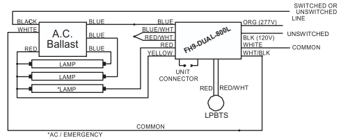
9. THREE LAMP INSTANT START BALLAST
