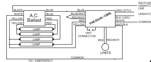
10. FOUR LAMP INSTANT START BALLAST
